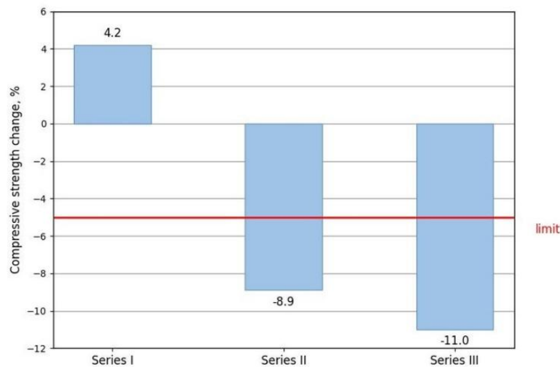
Fig. 3. Change in concrete compressive strength after 200 freezing and thawing cycles
