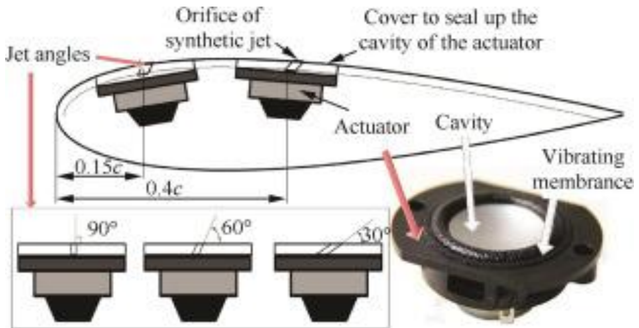
Fig. 5. Actuator concepts [5]
