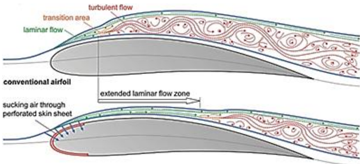
Fig. 1. HLFC – Hybrid Laminar Flow Control [3]
