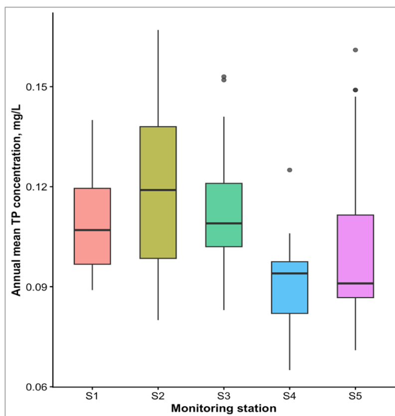
Fig. 3. Annual mean total phosphorus (TP) concentration at Nemunas River monitoring stations during 2001–2024
