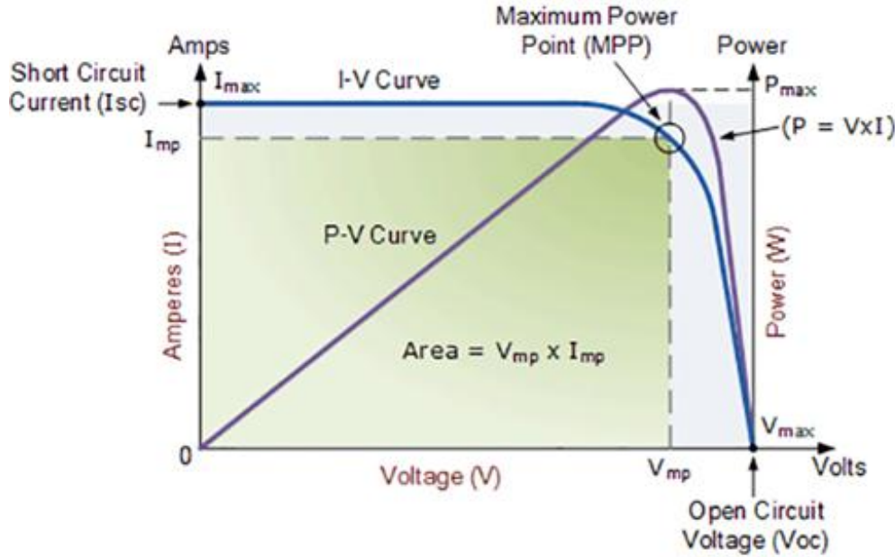
Fig. 1. Key Parameters of a Photovoltaic Module. Resources.
