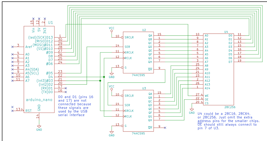
Fig. 4. Arduino-based EEPROM programmer schematic
