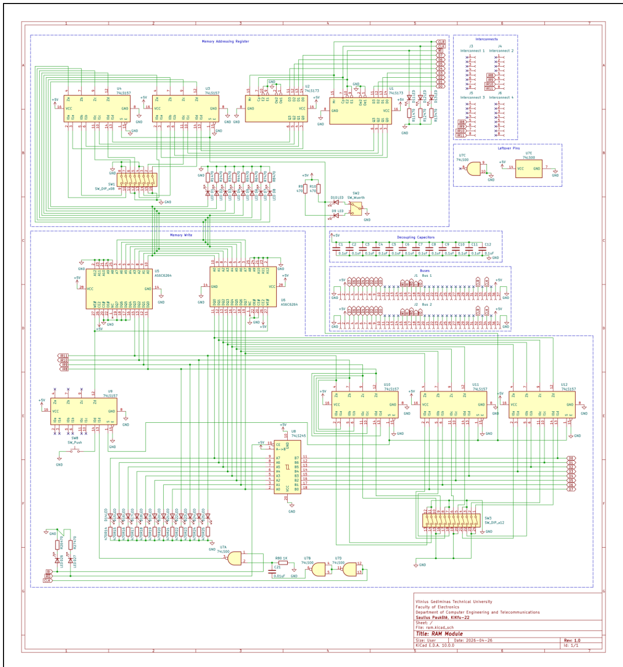
Fig. 11 pav. MAR and RAM schematic
