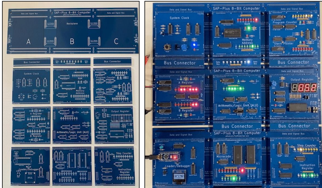
Fig. 6. Component-less PCB (left) and working, assembled computer (right)
