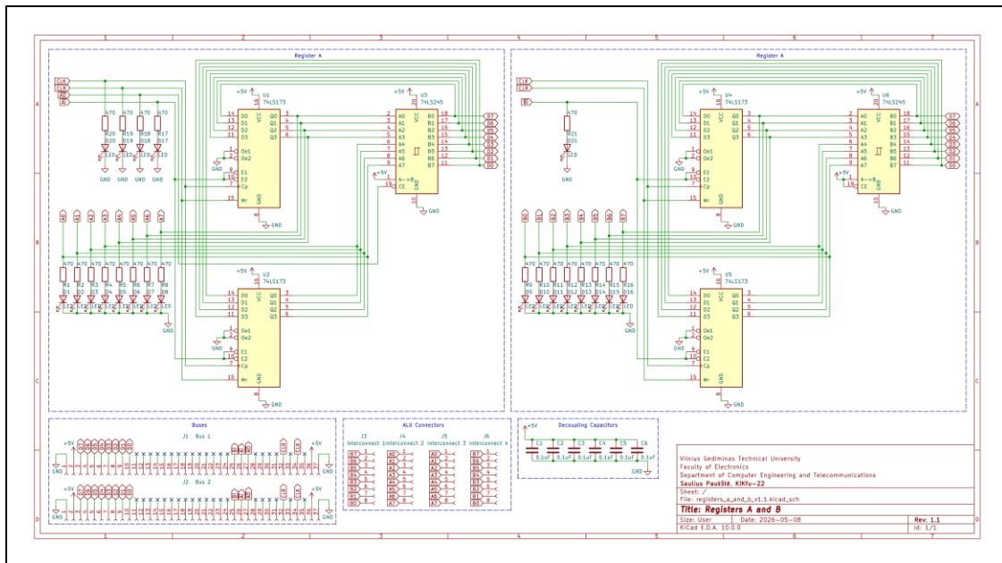
Fig. 12. Registers A and B schematic Source: made by author
