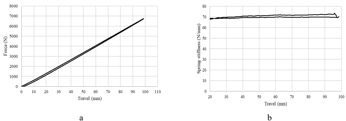
Fig. 2. Mechanical response of the (S2) rear axle coil springs: (a) force–displacement characteristics; (b) spring stiffness versus compression stroke
