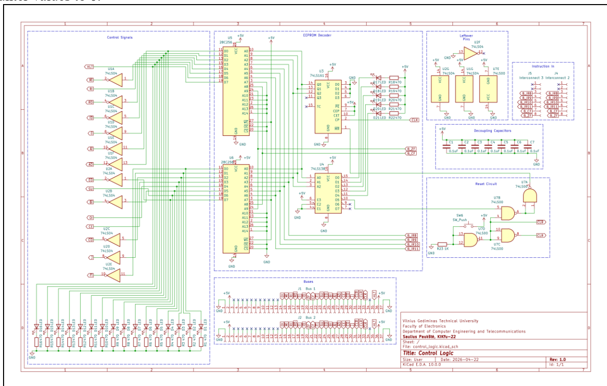
Fig. 9. Control logic schematic Source: made by author
