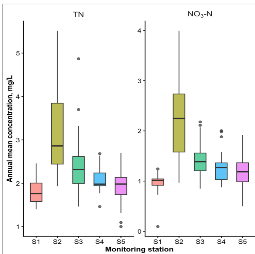
Fig. 2. Annual mean concentrations of total nitrogen (TN) and nitrate nitrogen (NO 3 -N) at Nemunas River monitoring stations during 2001–2024
