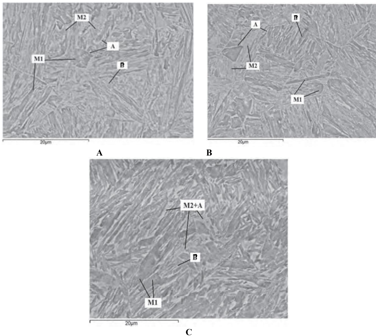
Fig.1. A.B and C. Microstructure of 20CrMn4 steel after different step-quenching variants (scanning electron microscopy): (M1 – primary martensite; B – bainite; M2 – secondary martensite; A – retained austenite)
