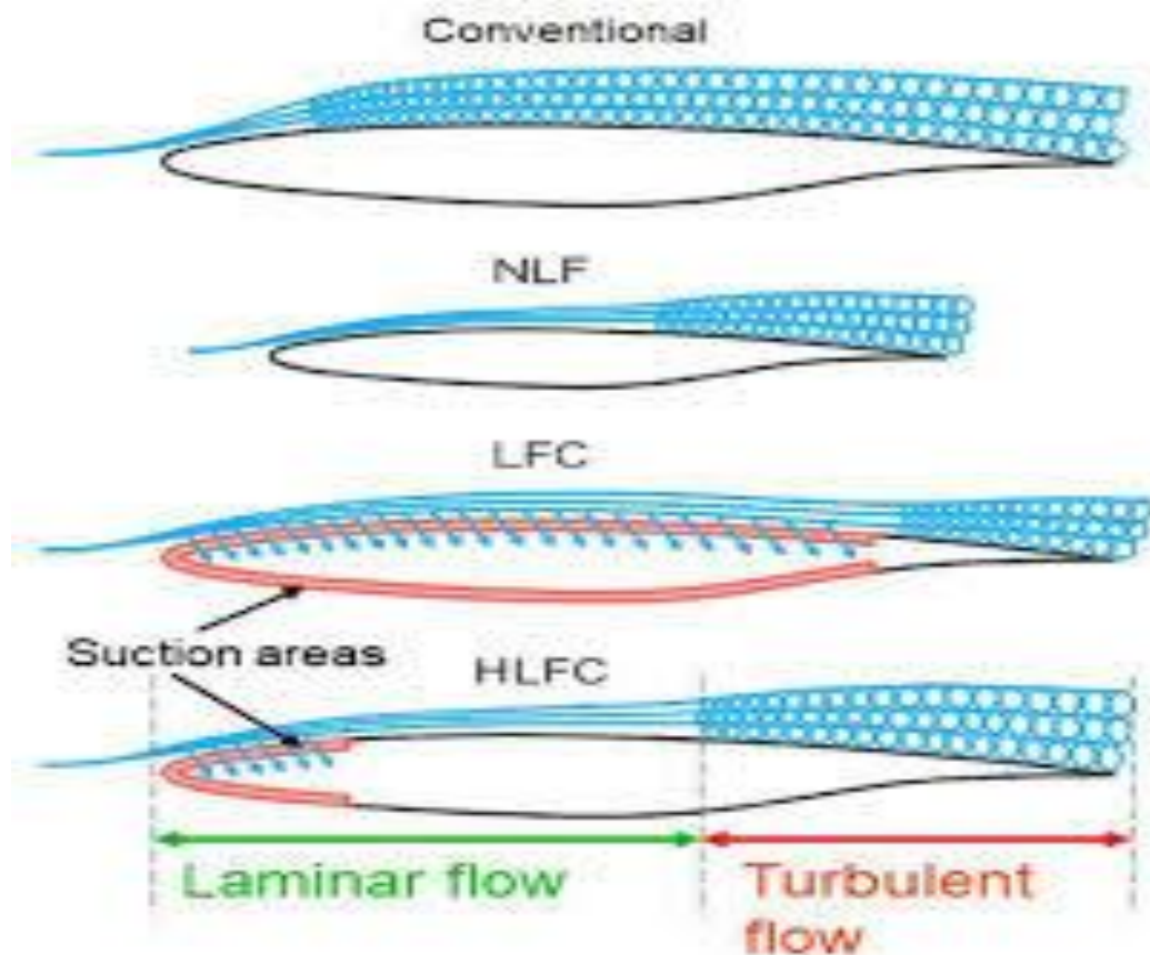
Fig. 4. Flow control for boundary layer separation [4]
