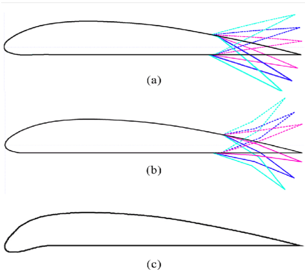
Fig. 3. The airfoil with traditional (a) and adaptive (b) mechanization. (c) The airfoil with an adaptive slat [5]
