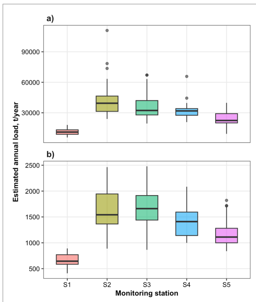
Fig. 4. Estimated annual loads of total nitrogen (a) and total phosphorus (b) at Nemunas River monitoring stations during 2001–2024 Source: compiled by the authors
