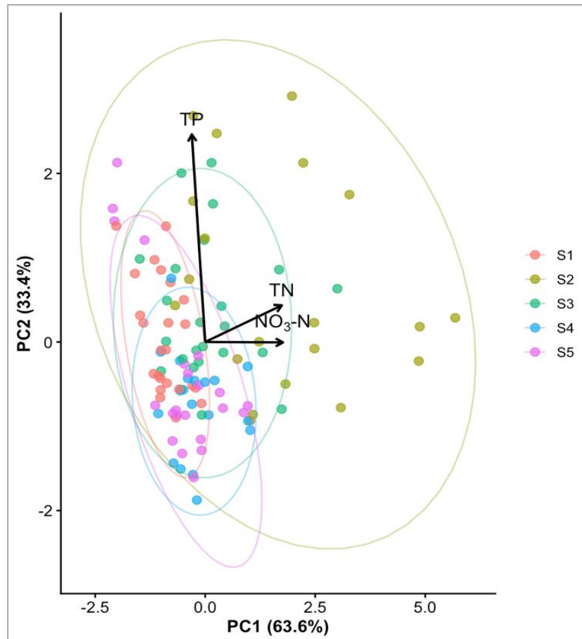
Fig. 5. PCA biplot of annual TN, \text{NO}_3\text{-N} and TP concentrations at Nemunas River monitoring stations during 2001–2024
