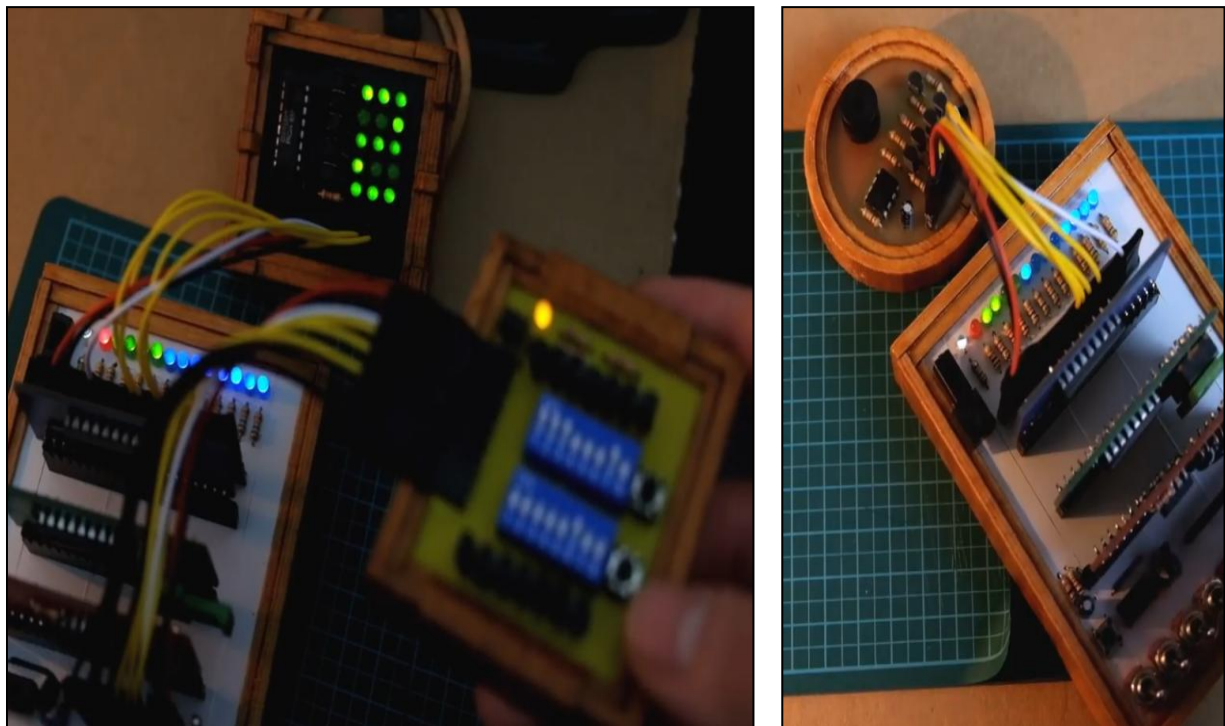
Fig. 2. 3x5 LED matrix and control input (left) and speaker (right) modules
