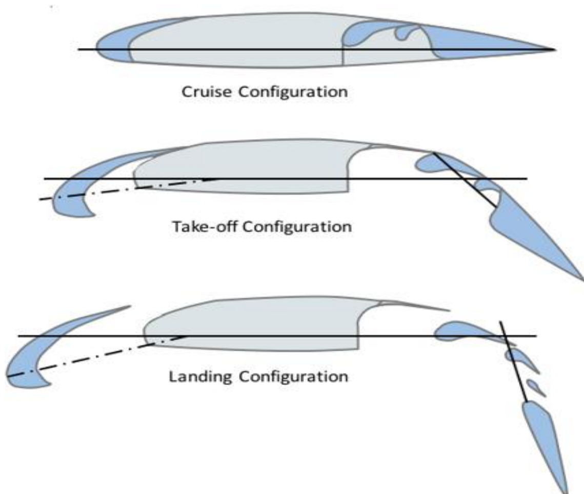
Fig. 2. Aircraft High-Lift System [4]
