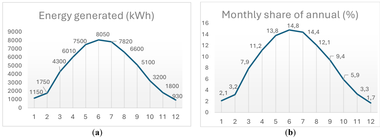
Fig.3. PV energy generation (kWh) and share of annual output: (a) Monthly energy output; (b) Monthly share of annual production.
