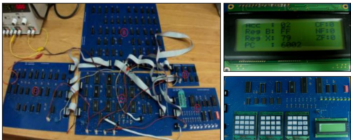
Fig. 5. ARC computer (left), where a – control unit, b – register connections, c – ALU, d – instruction decoder, e – external memory IO ports, and monitor with keypad control (right)
