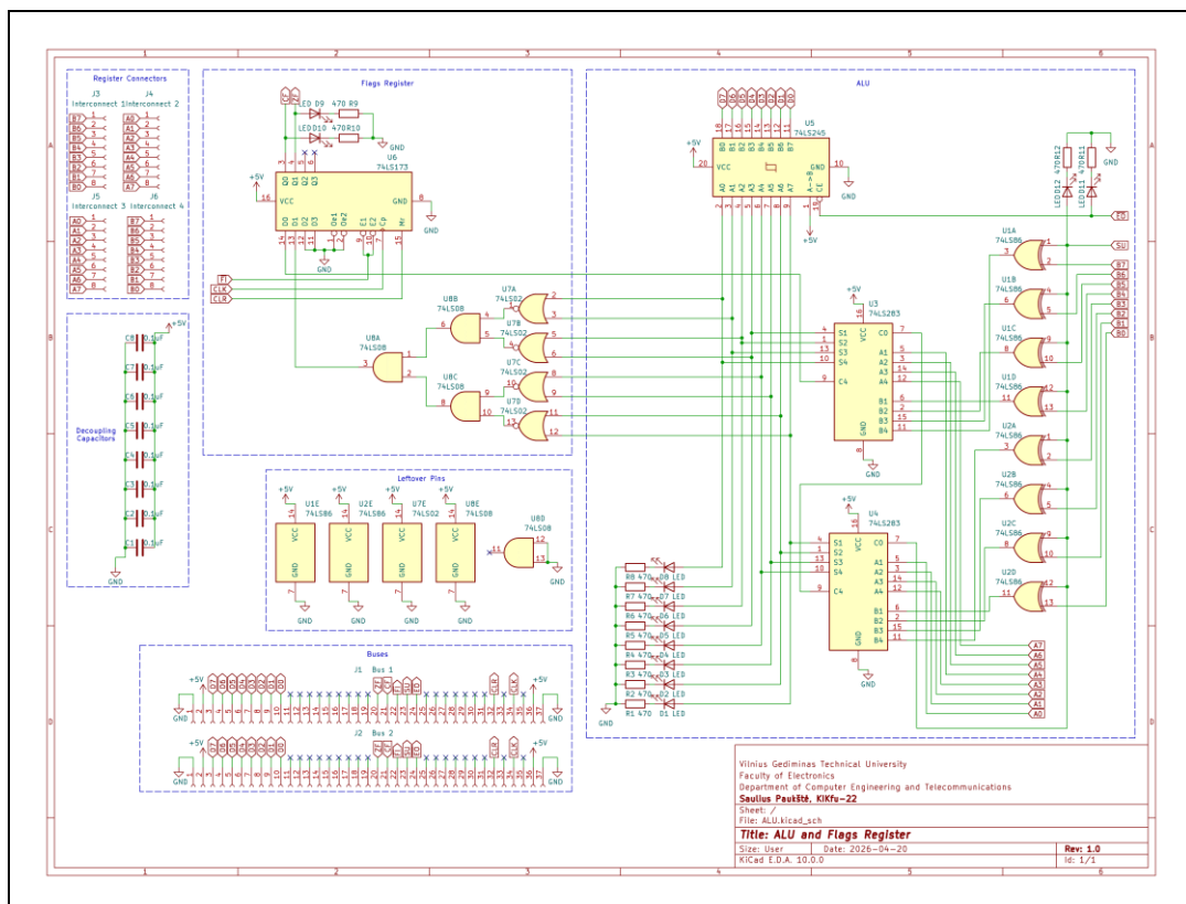
Fig. 13. ALU schematic Source: made by author
