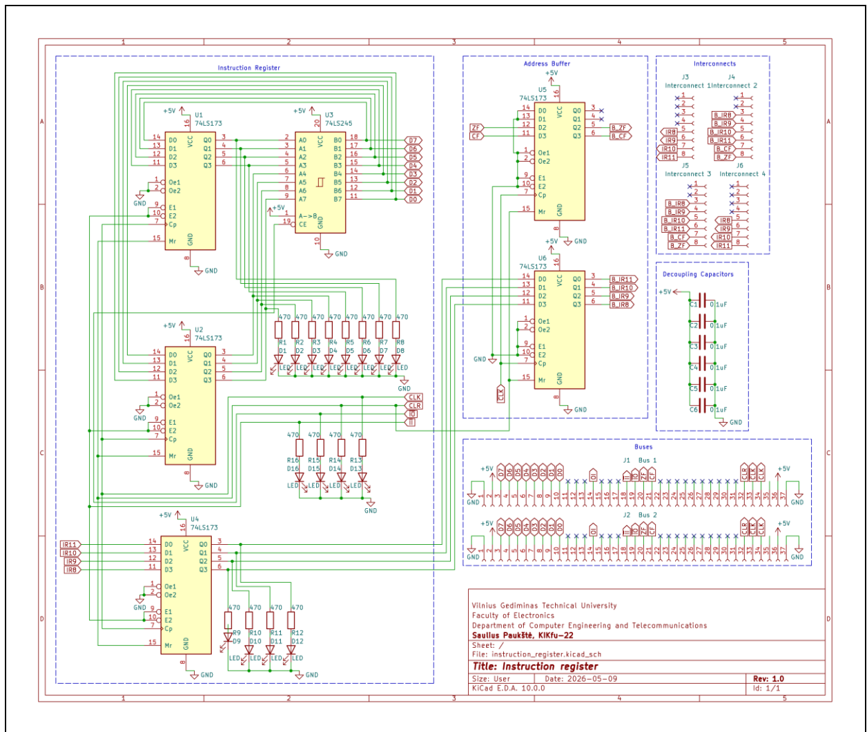
10 pav. Instruction register schematic
