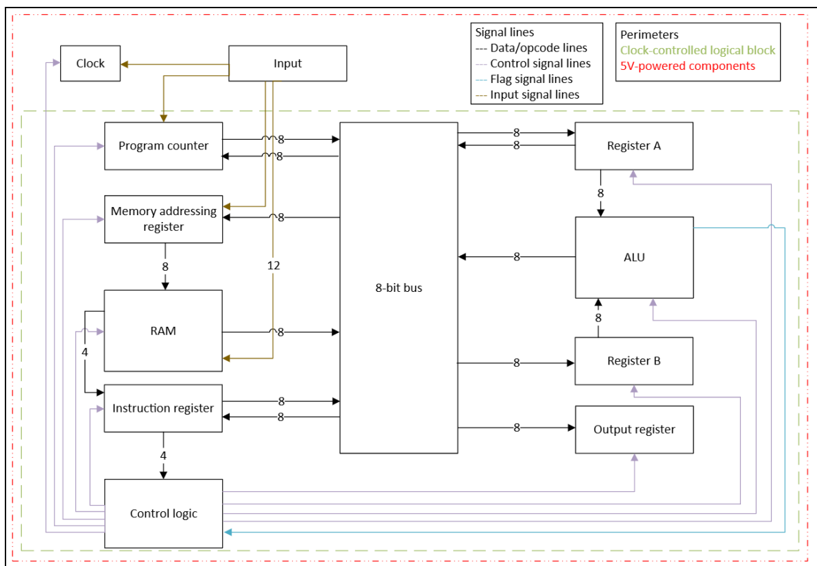
Fig. 7. Proposed functional block diagram for developed system
