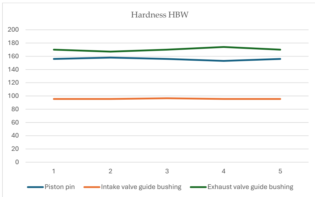
Figure 2. Hardness measurements of engine M-14P component materials
