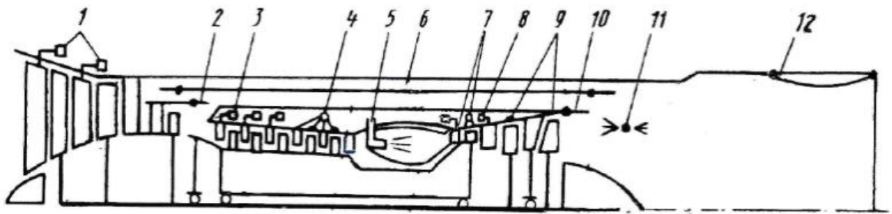
Fig. 15. Schematic of a hypothetical adaptive gas-turbine engine (GTE) with flow-path regulation elements
