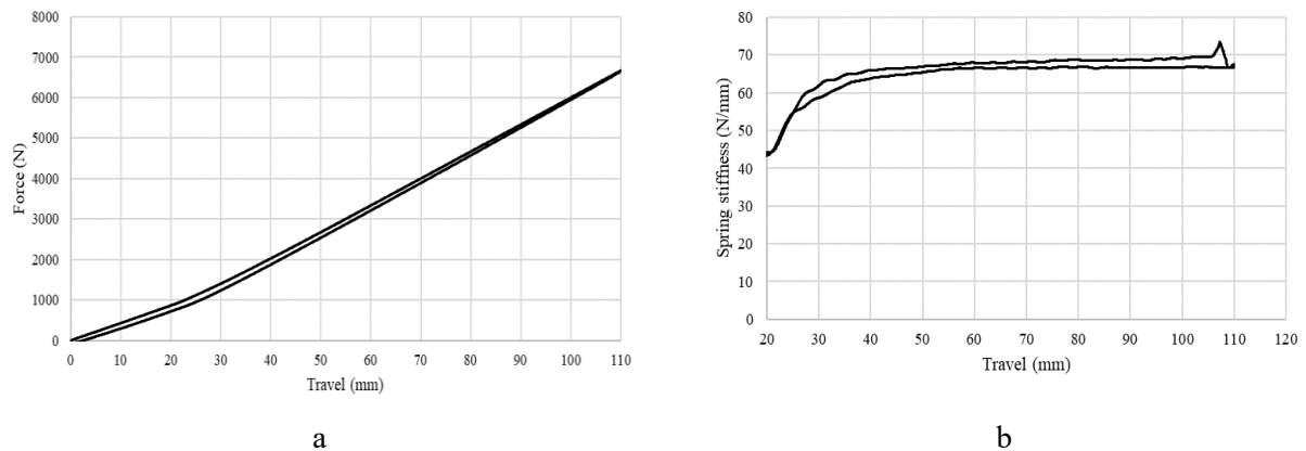
Fig. 1. Mechanical response of the (S1) rear axle coil springs: (a) force–displacement characteristics; (b) spring stiffness versus compression stroke
